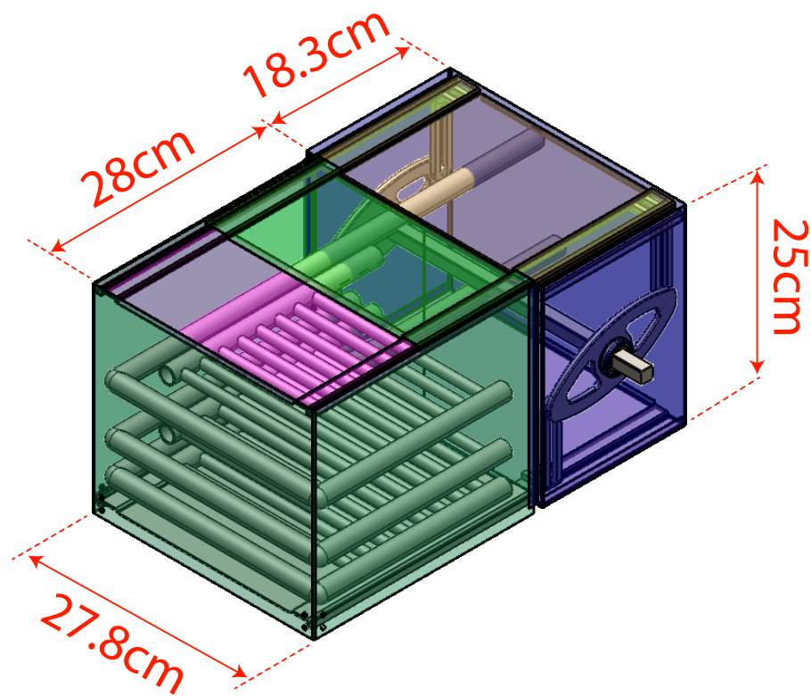
Heat Exchanger Provision with controlling Mechanism
