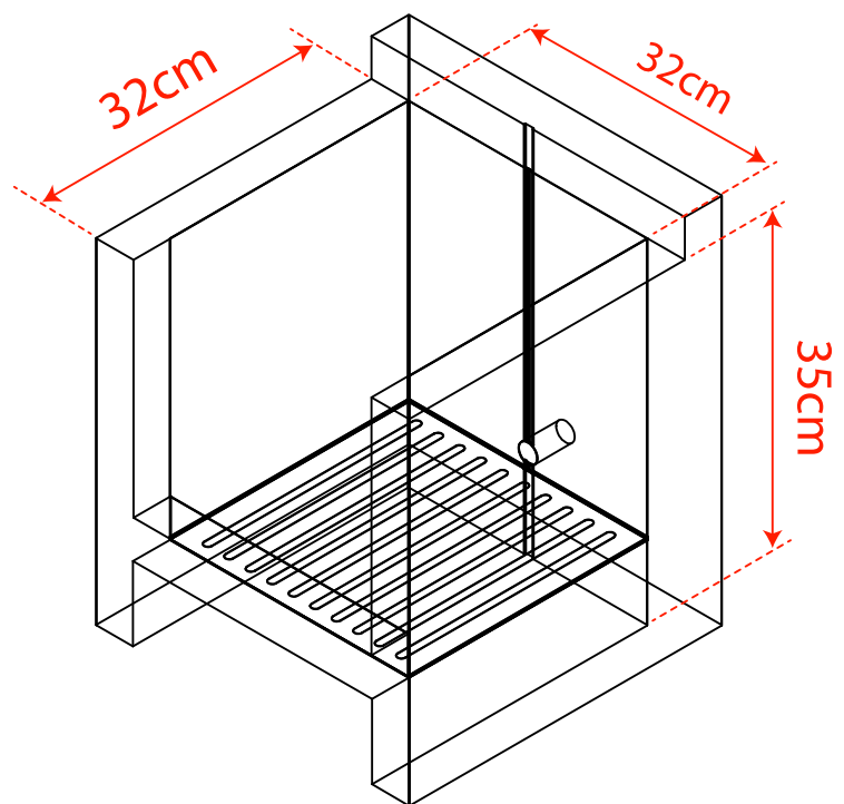
Combustion chamber
