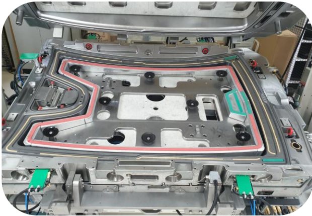
Encapsulation molds
